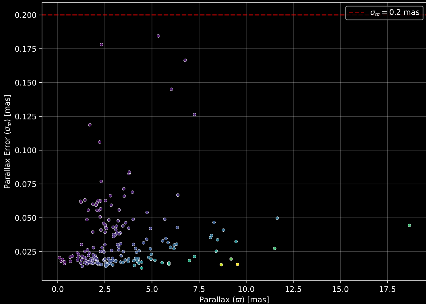
APOGEE DR17 Field: [K2_C3_045-54] Parallax Quality (n= 196)
