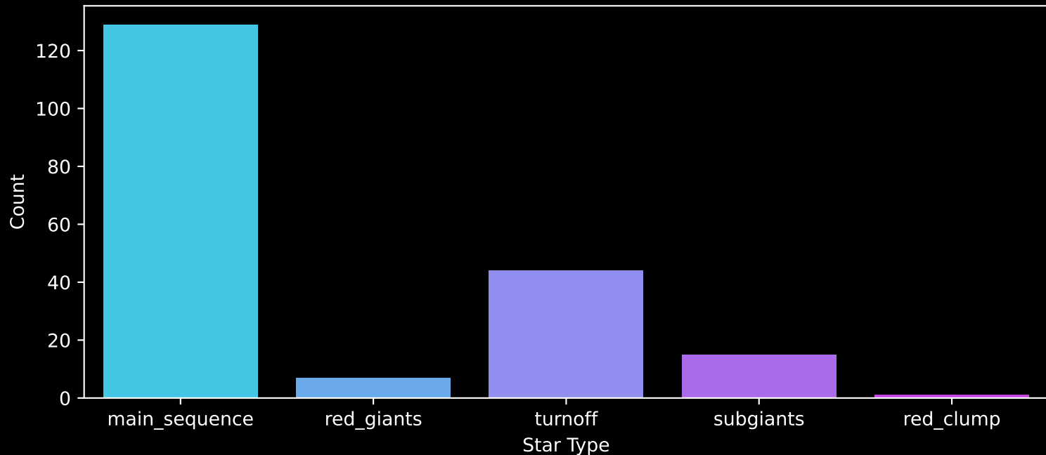
APOGEE DR17 Field: [K2_C3_045-54] Count plot of Star Type
