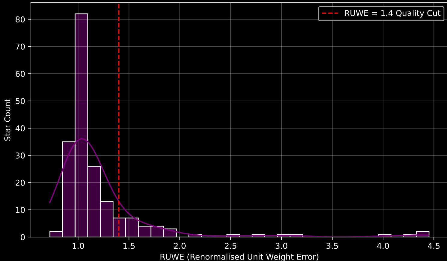
GAPOGEE DR17 Field [K2_C3_045-54] RUWE Distribution (n= 192)
