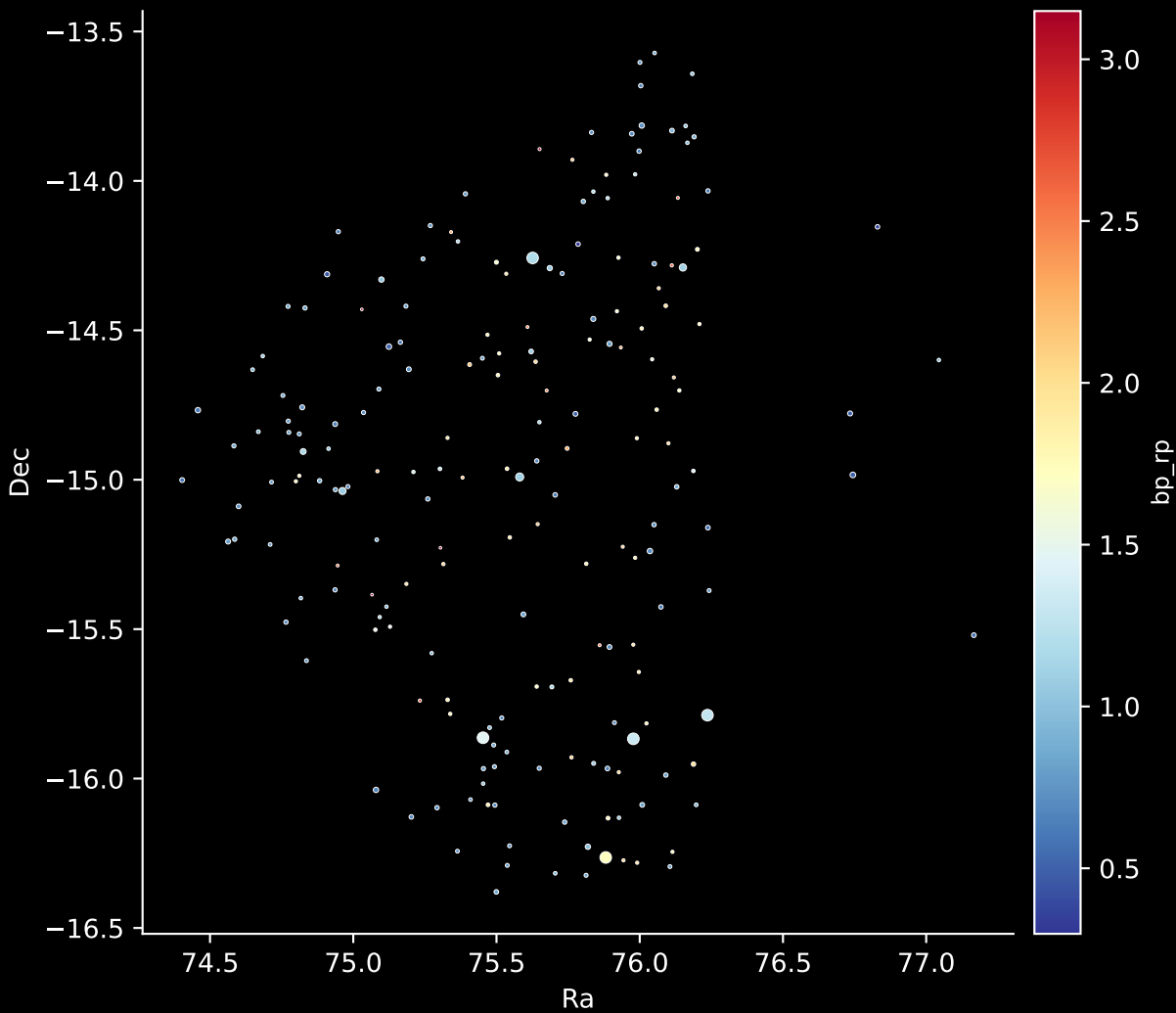
APOGEE DR17 Field: [K2_C3_045-54] Stars: 196
