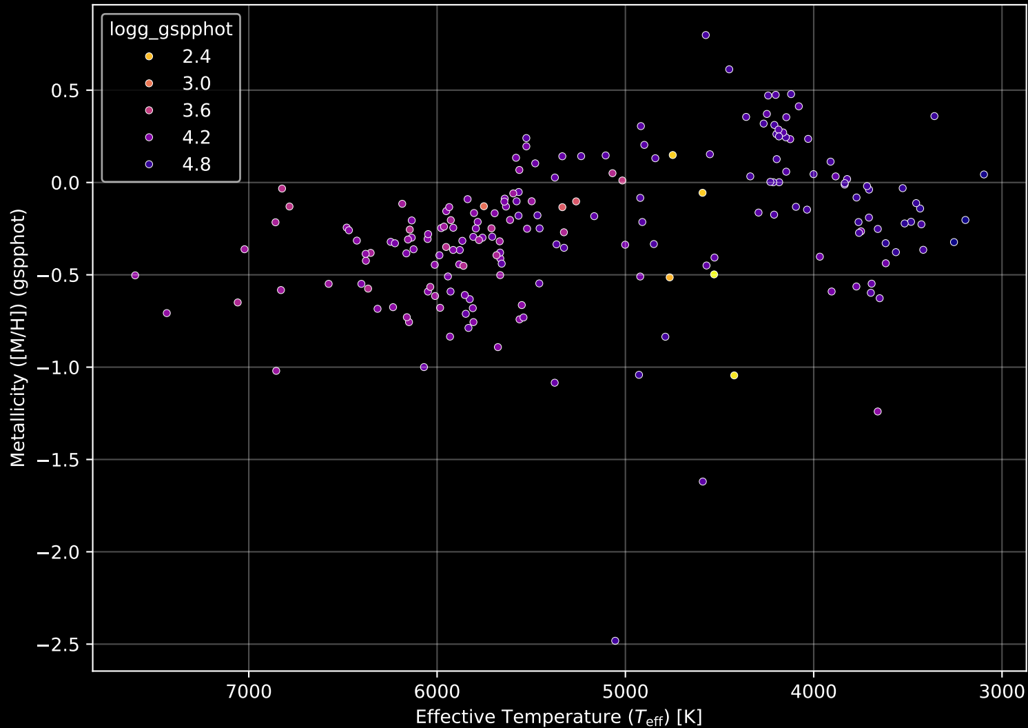
APOGEE DR17 Field: [K2_C3_045-54] Stellar Population Parameters (n= 196)
