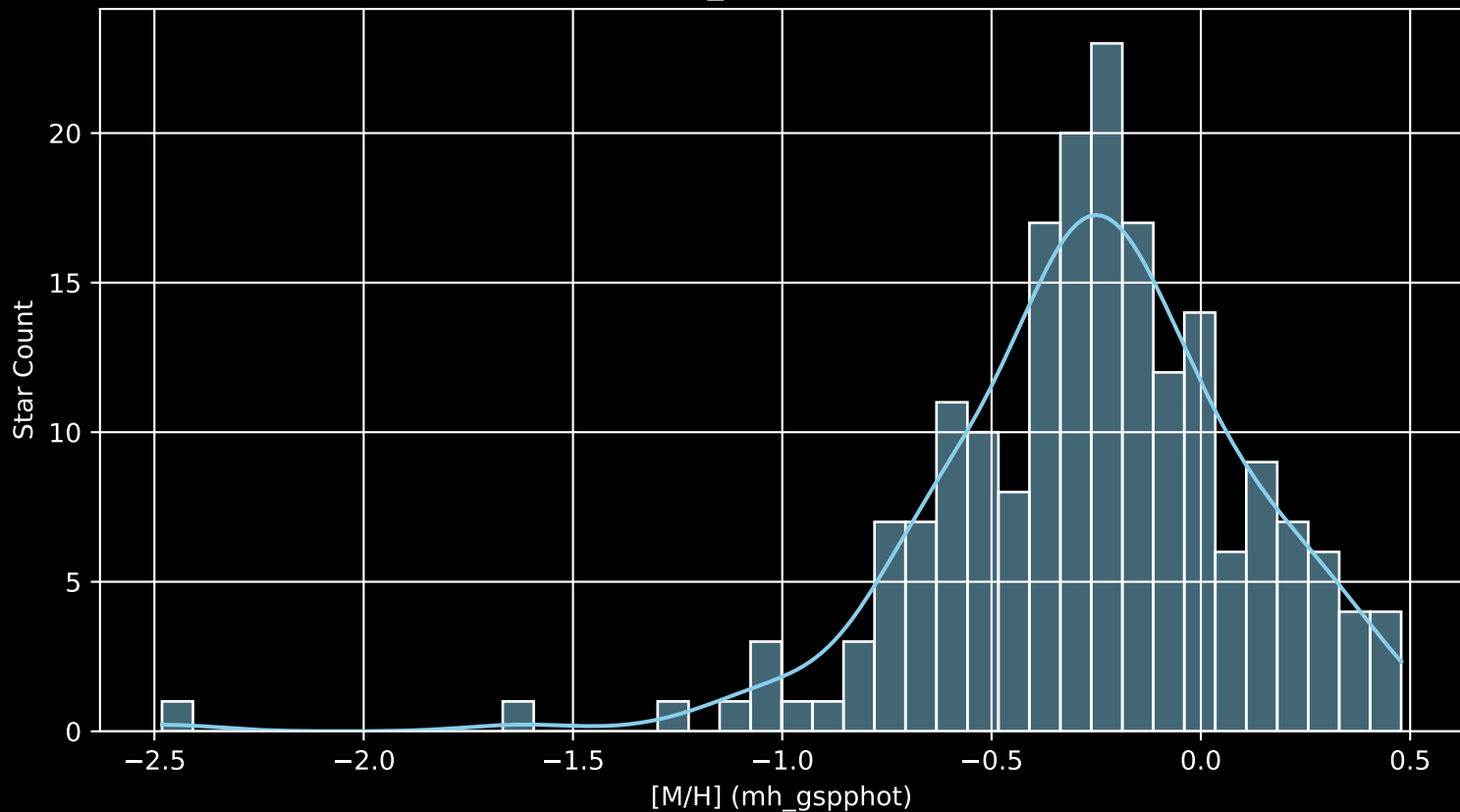
APOGEE DR17 Field: [K2_C3_045-54 [M/H] (mh_gspphot) (n= 194)
