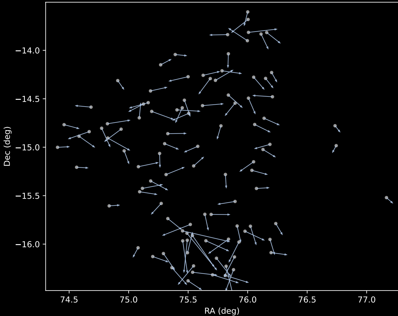
APOGEE DR17 Cluster 1 Proper Motion Vectors (n=101)
