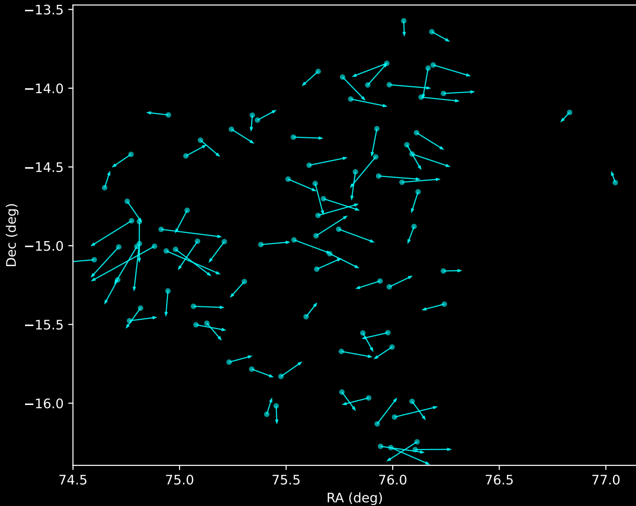
APOGEE DR17 Noise Stream Proper Motion Vectors (n=89)
