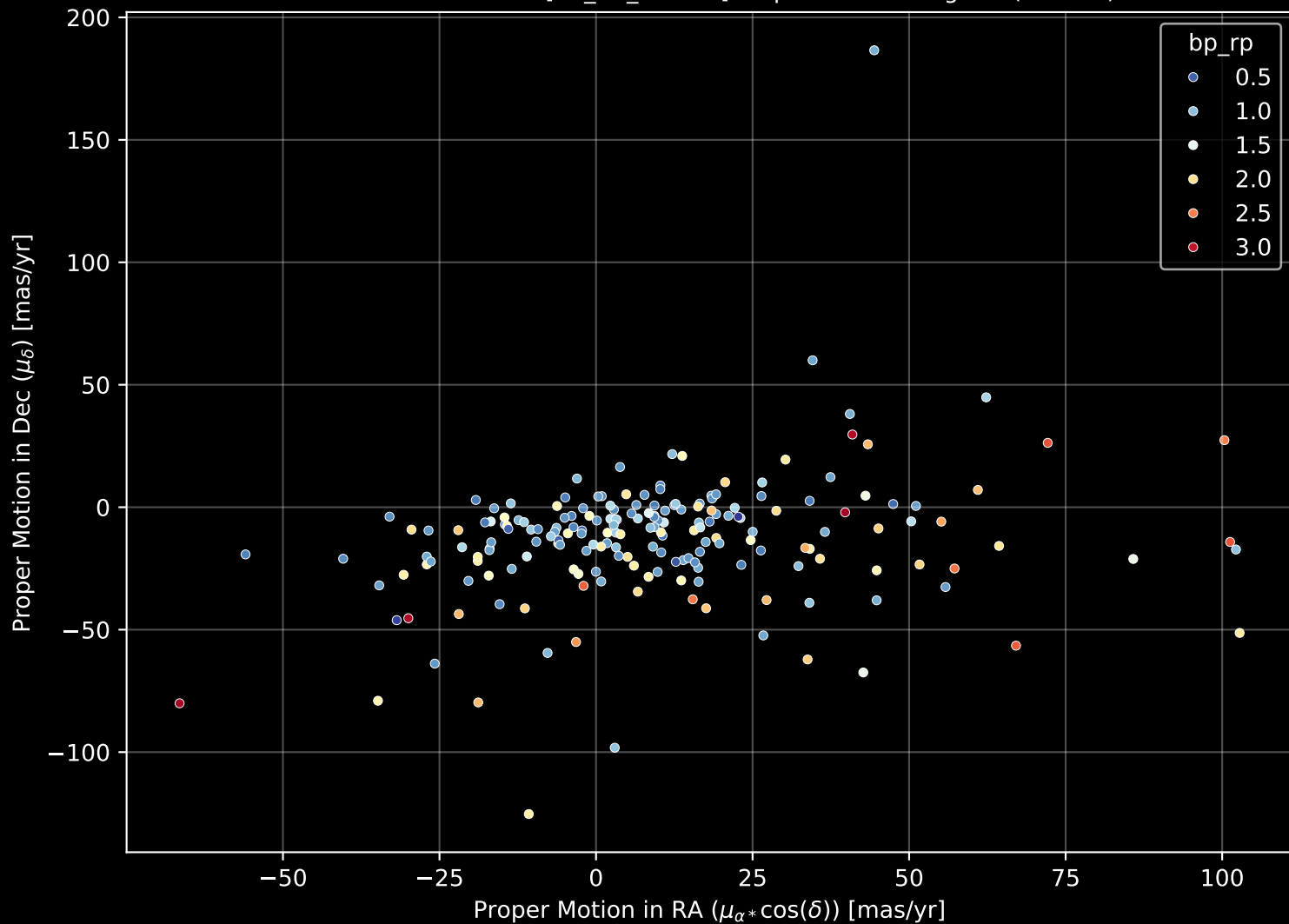
APOGEE DR17 Field: [K2_C3_045-54] Proper Motion Diagram (n= 196)
